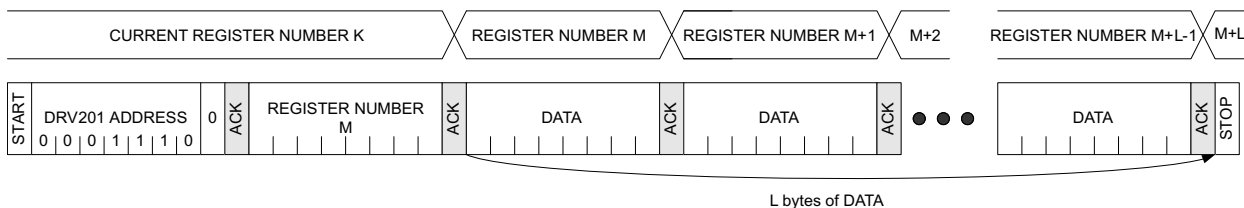
Figure 11. Sequential Write
